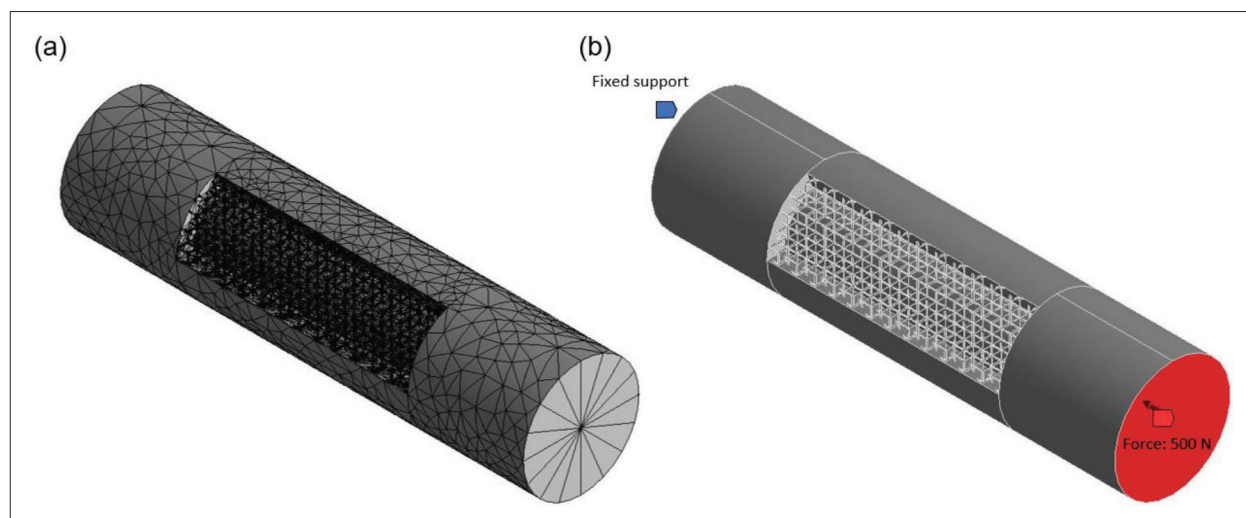
Figure 3. Boundary conditions for FEA results of hybrid structure with volume fraction 10%. (a) Mesh generation. (b) Fixed support and load conditions.
